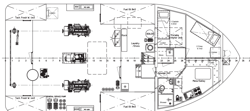
BELOW MAINDECK
